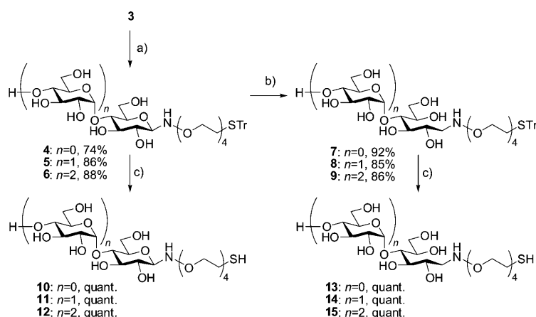
Scheme 3. Preparation of OEG glycoconjugates 4–6 by oxime coupling and subsequent reduction to oxyamines 7–9 . Removal of the trityl groups furnished thiol glycoconjugates 10–15 for coupling with gold nanoparticles. Carbohydrate oximes are depicted as the \beta -pyranose tautomer for the sake of clarity (Scheme 1). a) Glucose/maltose/maltotriose (1.1 equiv), MeCN, H 2 O, HOAc, 16 h; b) NaBH 3 CN (2 equiv), HOAc, 2 h; c) TFA, triethylsilane (TES), CH 2 Cl 2 , 5 min.
