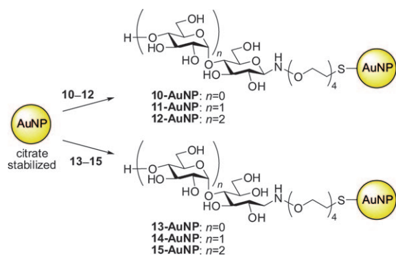
Scheme 4. Preparation of glyconanoparticles 10-AuNP to 15-AuNP . Carbohydrate oximes are depicted as the \beta -pyranose tautomer for the sake of clarity (Scheme 1).
