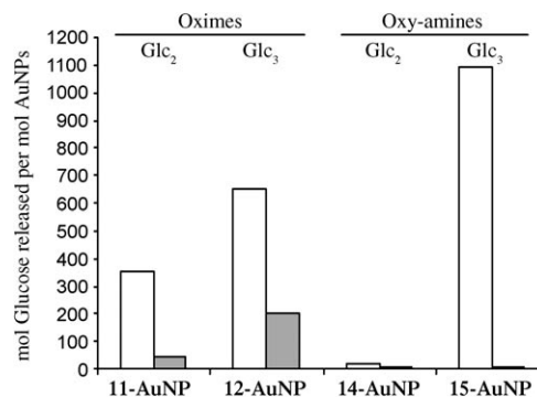
Figure 3. Measurements of release of glucose by glucoamylase after thiolytic release of OEG glycoconjugates from glyco-AuNPs (white bars) and by glucoamylase on glyco-AuNPs (grey bars). The experiment was performed in 10 mM sodium phosphate pH 7.0 at 42 °C using 50 pmol of each glyco-AuNP. As expected, 14-AuNP showed no response after thiolytic release (Table 2).
