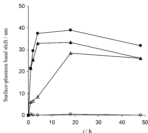
Figure 2. Lectin-induced nanoparticle aggregation as monitored by a shift in surface-plasmon band maximum for glyco-AuNPs 10-AuNP (●), 12-AuNP (▲), 13-AuNP (○), and 15-AuNP (△) upon addition of 5- \mu\text{M} concanavalin A.
