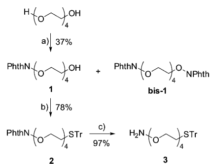
Scheme 2. Preparation of heterobifunctional aminooxy linker 3 from tetra(ethylene glycol). a) 1 equiv PhthN-OH, PS-PPh 3 , diisopropyl diazodicarboxylate (DIAD), 16 h; b) TrSH, PS-PPh 3 , DIAD, 0°C→RT, 16 h; c) hydrazine hydrate, MeCN, RT, 2 h.
