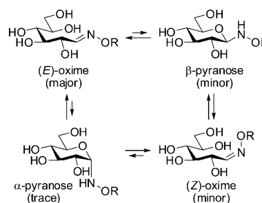
Scheme 1. Ring-chain tautomers of glucose oxime ethers. Adapted from ref. [30].
